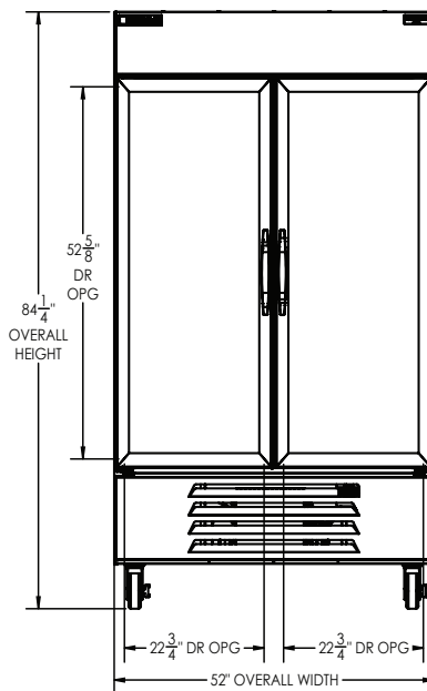
ELEVATION VIEW
