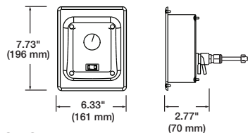
HBGB Optional Flush Mount Control Box
