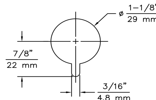
MOUNTING HOLE SCALE: 2/1
