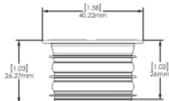
HOUSING WITH GASKET
