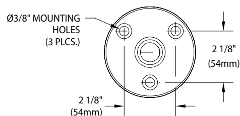
DETAIL "A" ALUMINUM WALL MOUNTING BRACKET
