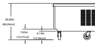
TYPICAL END
