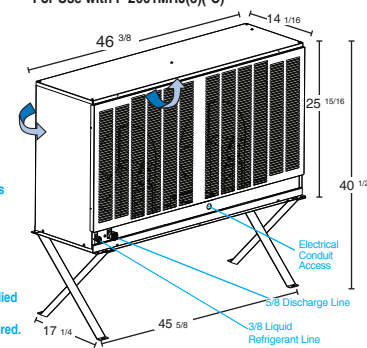
REMOTE AIR-COOLED
