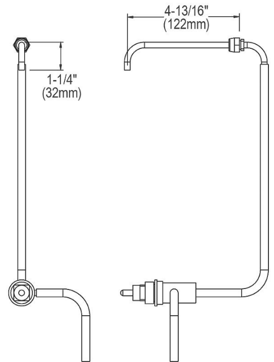
SOAP SPOUT
