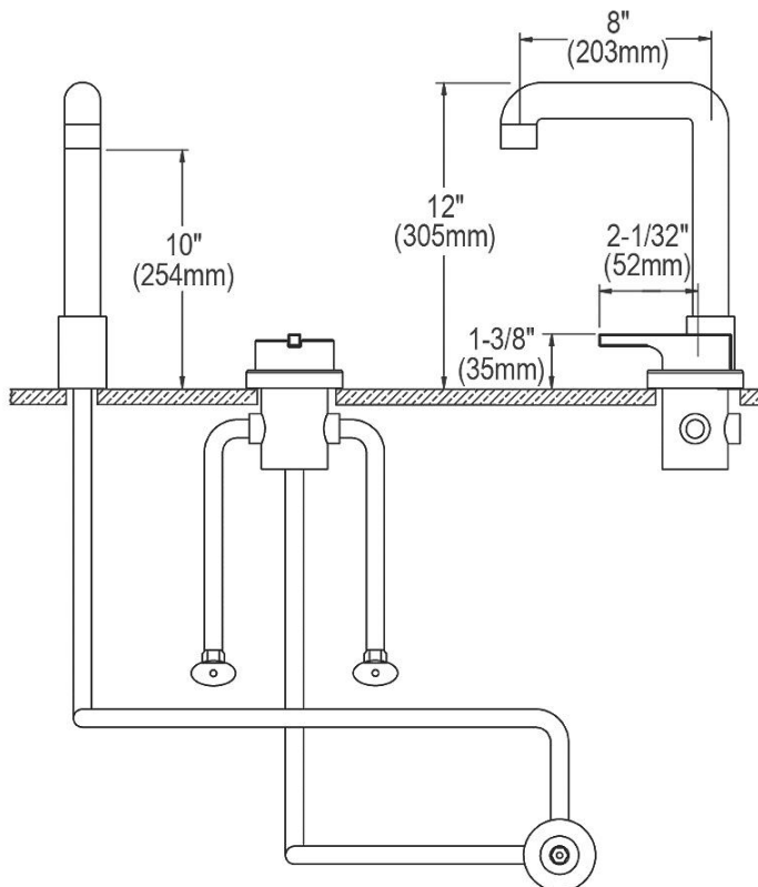
FAUCET AND TEMPERATURE HANDLE
