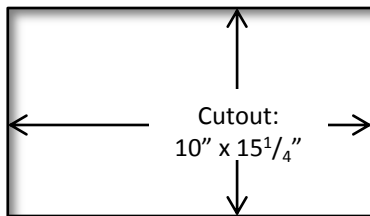
E1 Accessory cutout (Not to scale)
