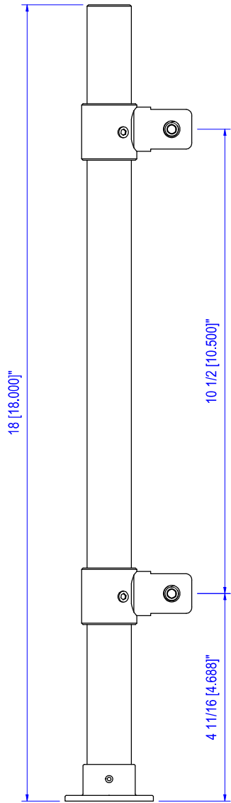
FRONT VIEW SNEEZEGUARD POLE (END)
