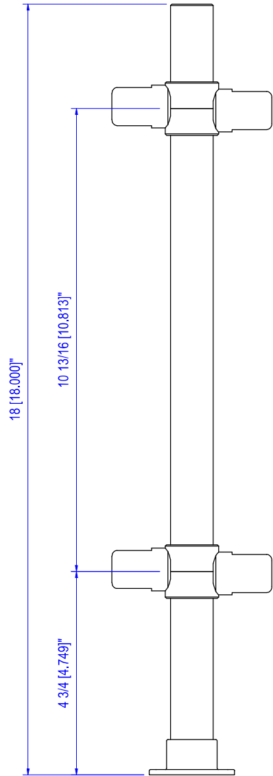
FRONT VIEW SNEEZE GUARD POLE (MID)
