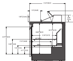
UC4460N-8 Right Side View
