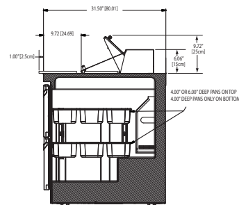
UCD4460N-8 Right Side View
