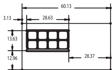
UC4460N-8 Pan Cutout Configuration
