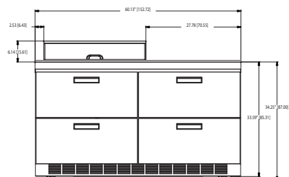
UCD4460N-8 Elevation View
