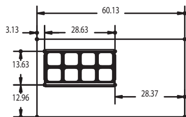
UCD4460N-8 Pan Cutout Configuration
