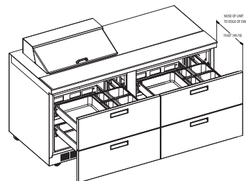
UCD4460N-8 ISO View
