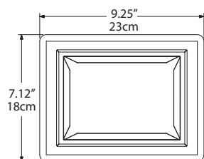
Plan View ND-57
