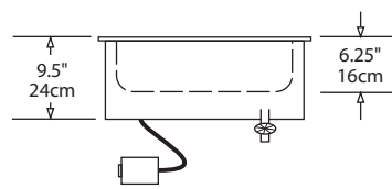
Right End View
