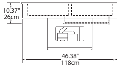
Elevation View 8148-EFN
