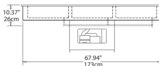
Elevation View 8169-EFN
