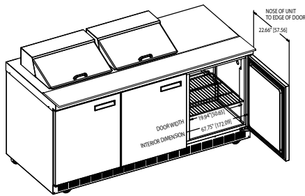
4472N-12 ISO View
