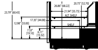
4472N-12 Elevation View
