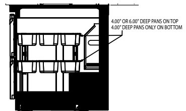
D4472N-12 Elevation View
