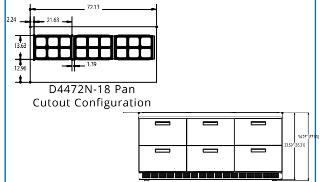
D4472N-18 Elevation View
