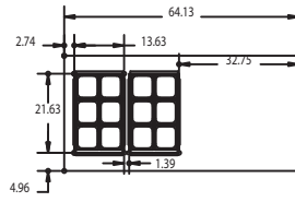
D4464N-12M Pan Cutout Configuration
