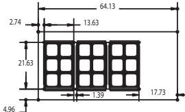
D4464N-18M Pan Cutout Configuration
