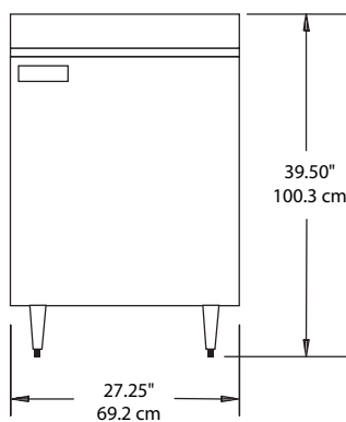
Elevation View 402/403
