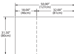
Plan View 18650VDL, 18650VDL-CE
