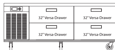
Elevation View 18682VDL, 18682VDL-CE
