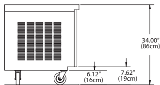
Left End View 18650VDL, 18650VDL-CE, 18682VDL, 18682VDL-CE
