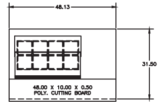
D4448NP-8 Pan Cutout Configuration
