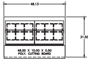
4448NP-12 Pan Cutout Configuration
