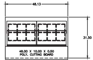
D4448NP-12 Pan Cutout Configuration
