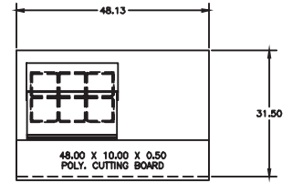
D4448NP-6 Pan Cutout Configuration
