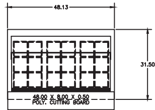
4448NP-18M Pan Cutout Configuration
