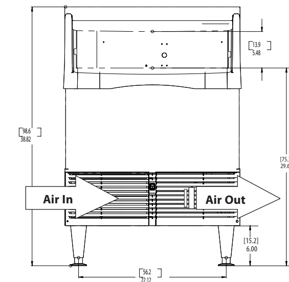
CU1526/CU2026 front view
