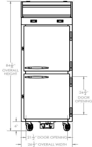
ELEVATION VIEW
