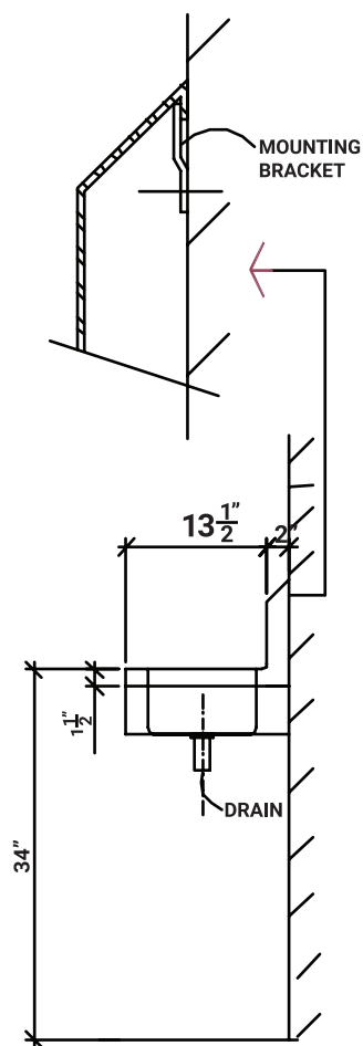
END VIEW
