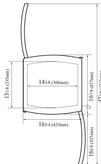
PLAN VIEW
