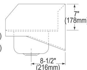
SECTION THROUGH RIM
