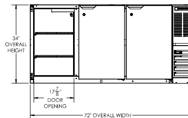
ELEVATION VIEW
