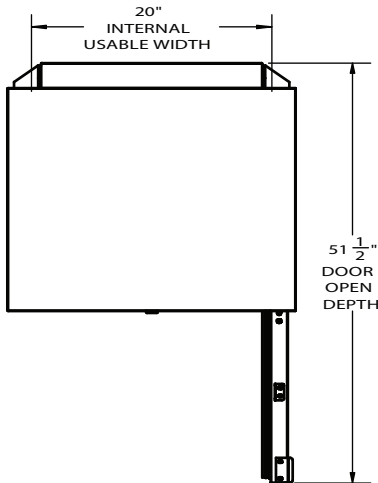
PLAN VIEW
