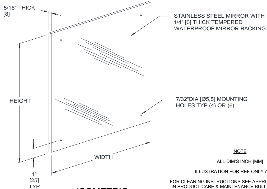
ISOMETRIC
