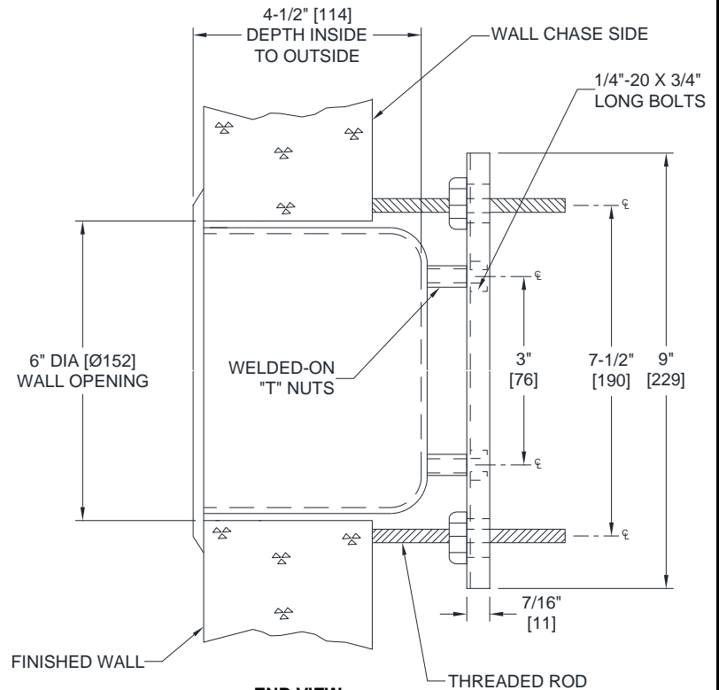
END VIEW
