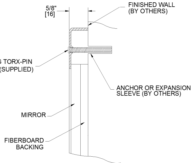
INSTALLATION DETAIL
