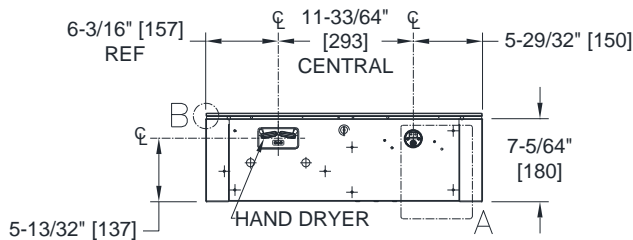
BOTTOM VIEW (-1, -2)
