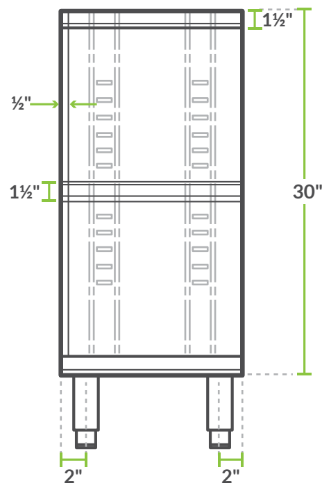
SIDE
