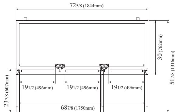
PLAN VIEW
