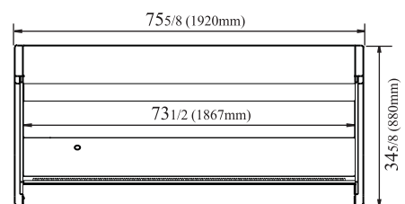
TOM-75S(B) TOP VIEW
