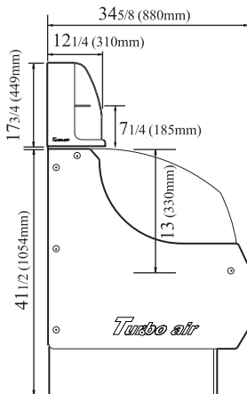
TOM-S w/ TOMD-H SIDE VIEW
