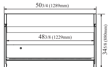
TOM-50S(B) TOP VIEW
