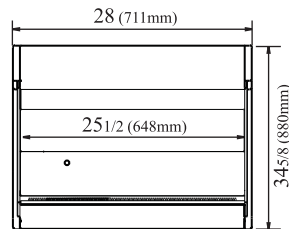
TOM-30S(B) TOP VIEW
