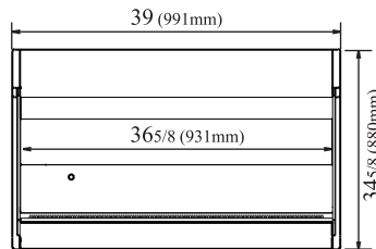
TOM-40S(B) TOP VIEW
