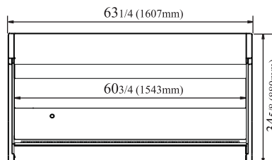
TOM-60S(B) TOP VIEW
