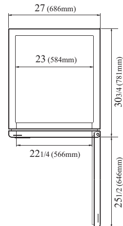
PLAN VIEW
