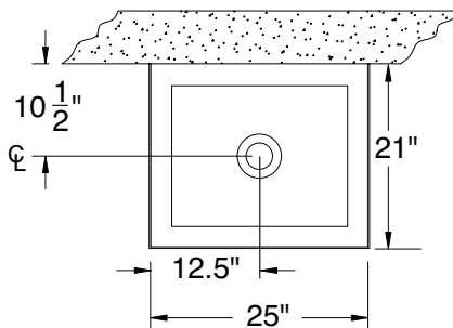
Mop Sink Detail
