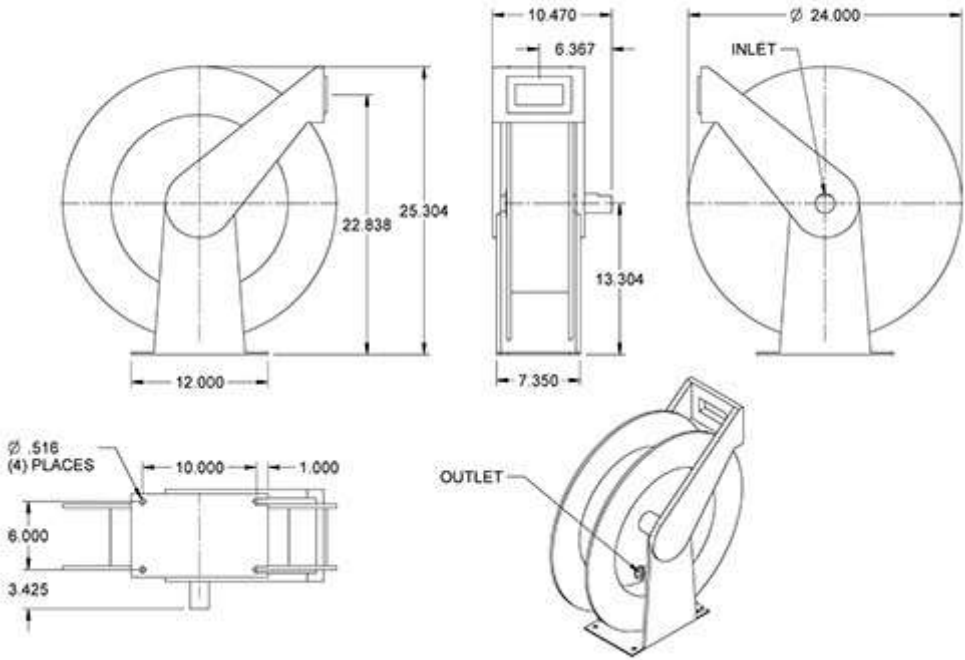
80000 OXP SW DIMENSIONAL DRAWING
