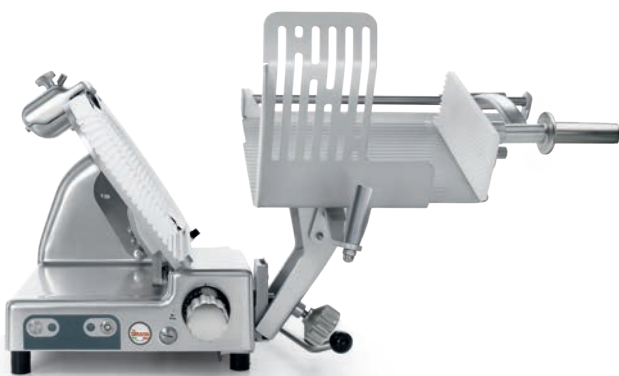
Tilt-carriage with zero blade exposure
