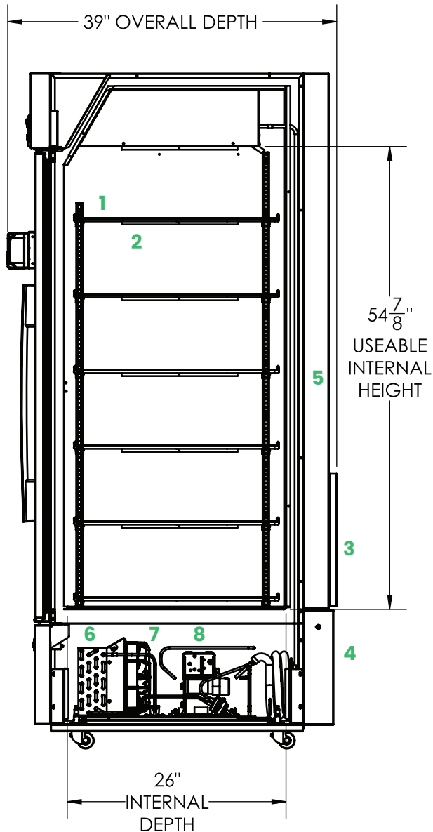
Internal Side View
