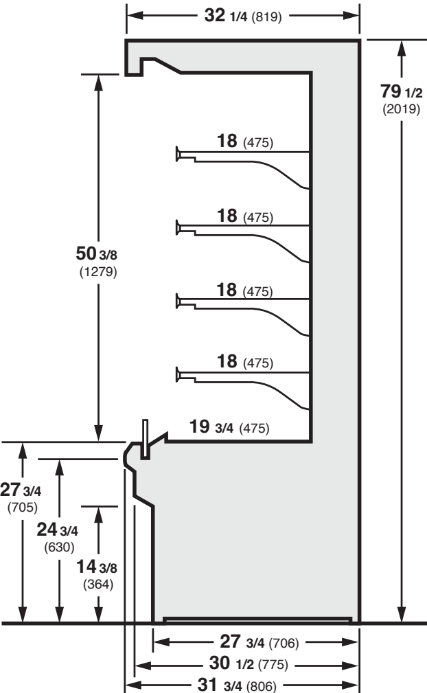
Cross Section
