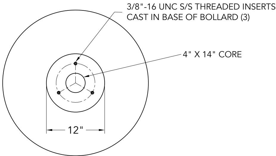
3 BOTTOM VIEW
