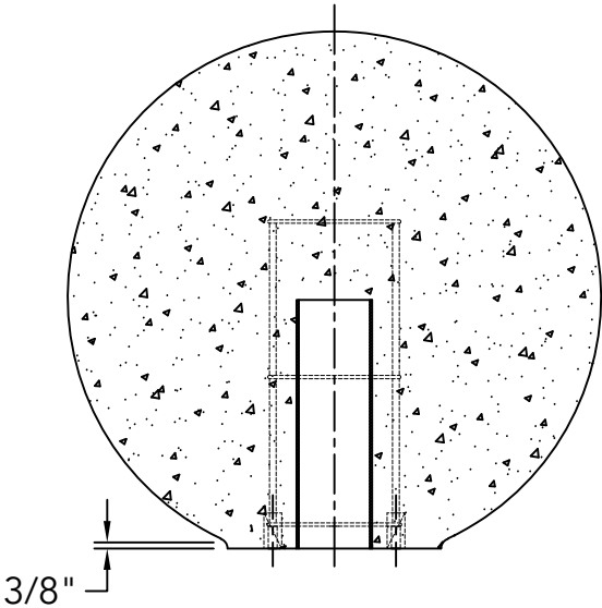
4 SECTION VIEW
