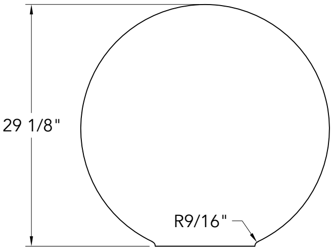
1 FRONT VIEW
