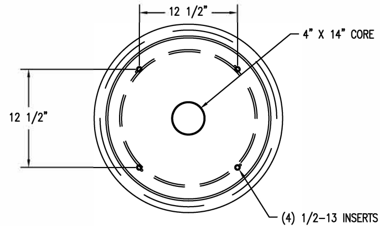
3 BOTTOM VIEW
