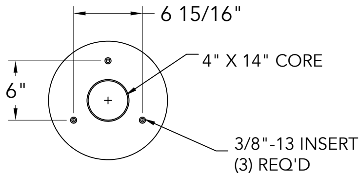
3 BOTTOM VIEW
