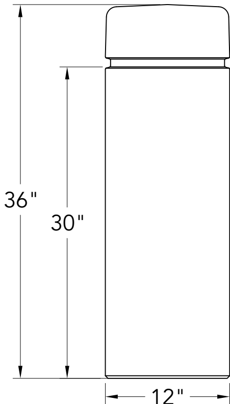
1 FRONT VIEW
