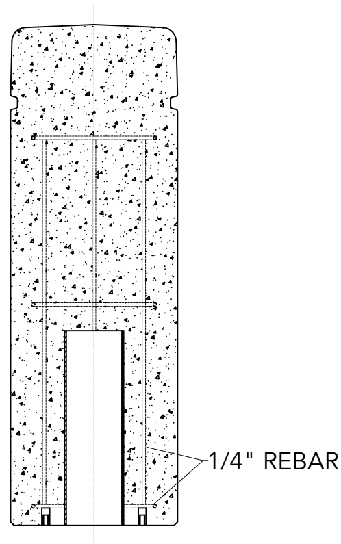
4 SECTION VIEW
