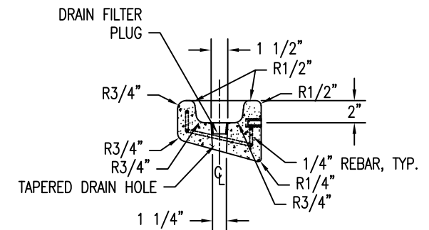
4 CROSS SECTION
