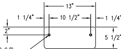
3 BACK VIEW OF TF2090 SNUFFER
