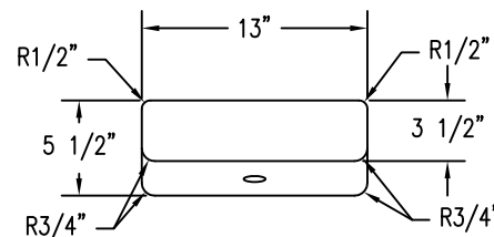
2 FRONT VIEW OF TF2090 SNUFFER
