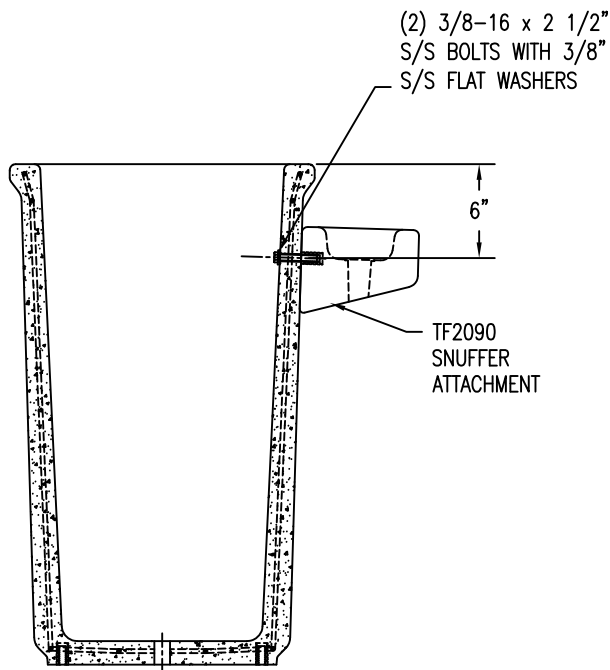
5 SNUFFER LOCATION ON W-19
