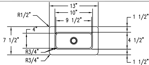
1 TOP VIEW OF TF2090 SNUFFER
