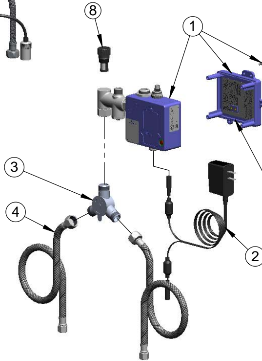
Optional 0.5 GPM VR Non-Aerated Spray Device Included
