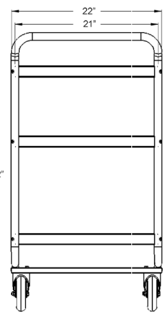
End View
