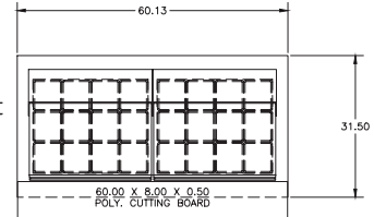
D4460NP-24M Pan Cutout Configuration
