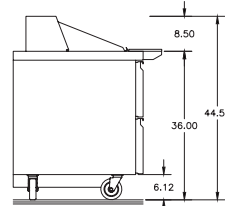
D4460NP-12M Right Side View
