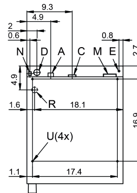
Connection points, bottom of unit
