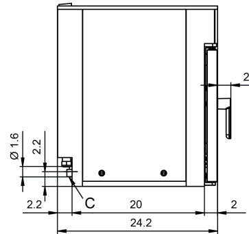
Connection points, bottom of unit
