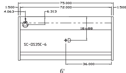
REMOTE - PLAN VIEWS
