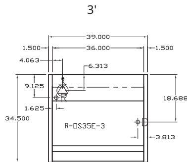
REMOTE - PLAN VIEWS
