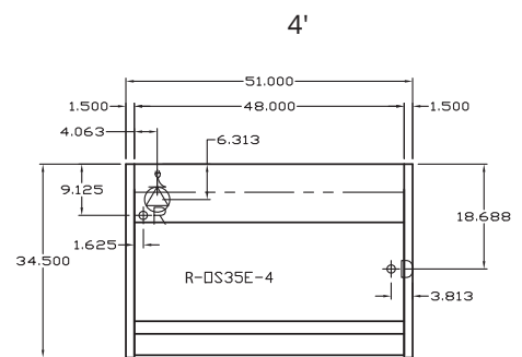
REMOTE - PLAN VIEWS
