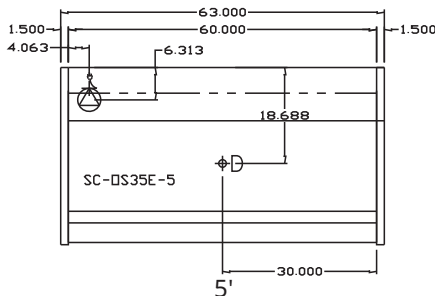
REMOTE - PLAN VIEWS
