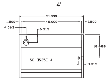
SC - PLAN VIEWS
